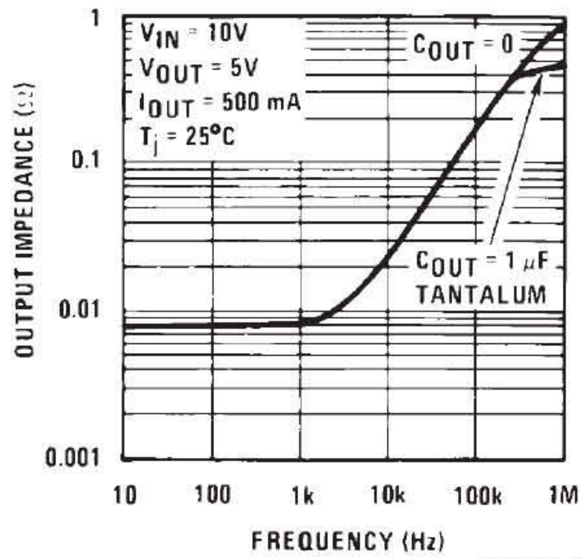
Output Impedance
