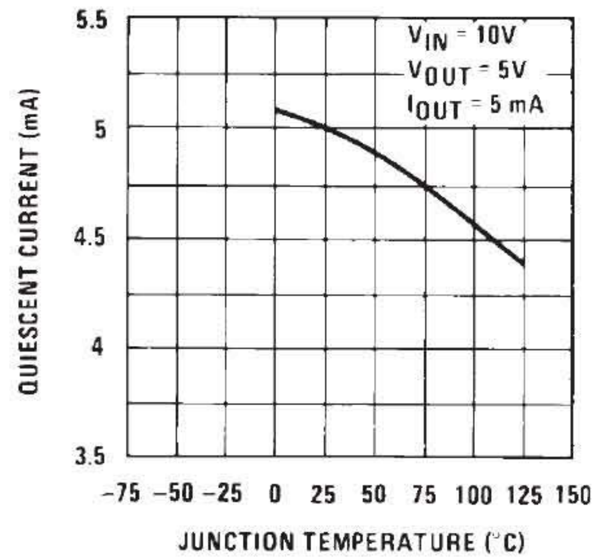
Quiescent Current
